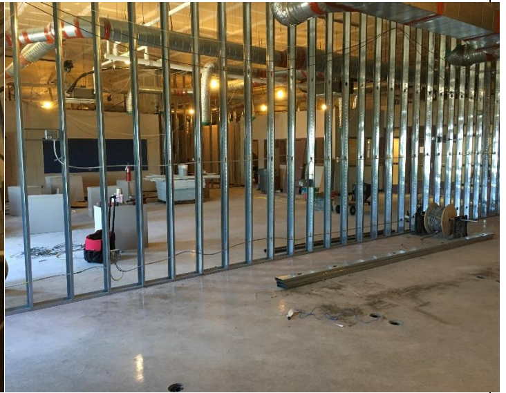
Rm. 228-232 New Wall Elec. Rough-In 7-19-18
